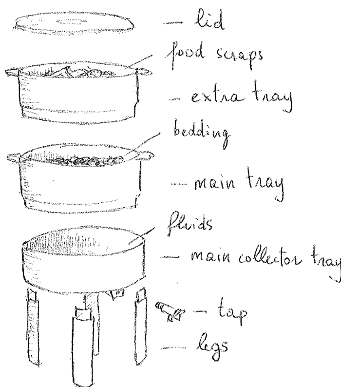
Figure 1 The various parts of the bin to be assembled. Drawn by the authors.
